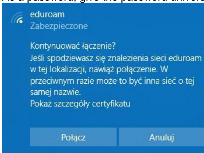
Figure 4: Warning Message
